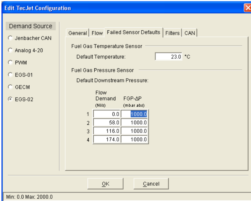
Figure 5-11. Edit TecJet Configuration, Failed Sensor Defaults
