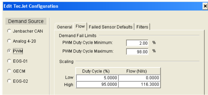
Figure 5-10c. Edit TecJet Configuration, Flow (PWM Demand)
