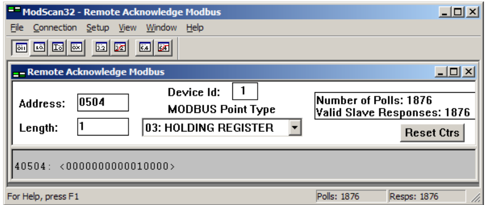
Figure 5-14: Modbus - remote control parameter 503
